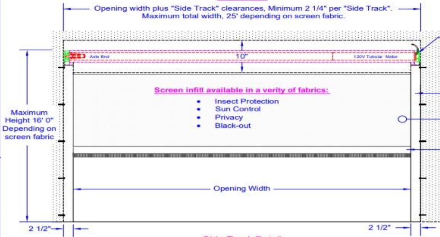
Side Track Detail
