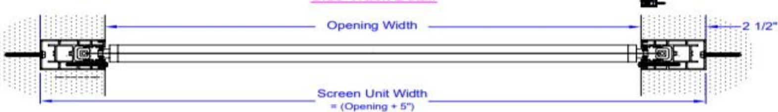
Side Track Detail
